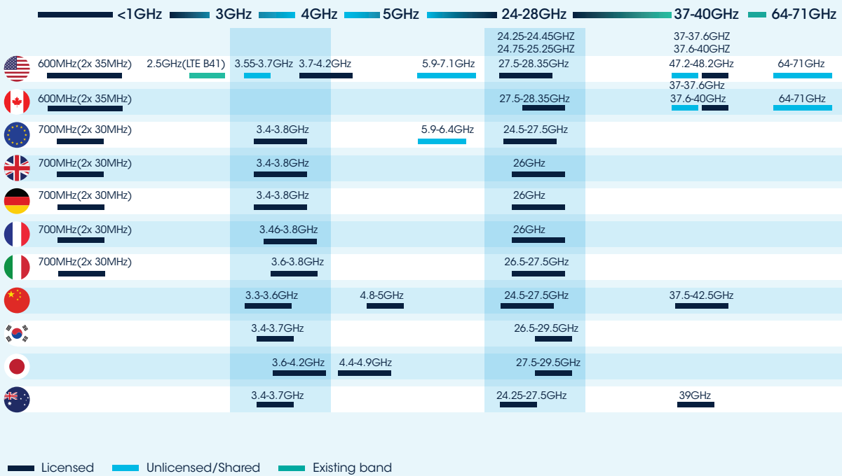
FIGURE 13: GLOBAL SNAPSHOT OF 5G SPECTRUM
