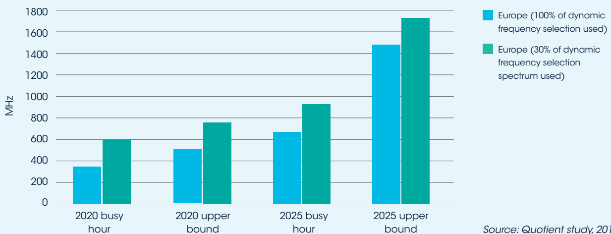
FIGURE 8: THE POTENTIAL SPECTRUM SHORTFALL IN EUROPE
