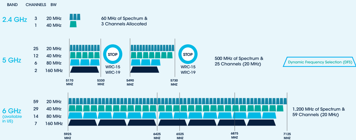
FIGURE 9: THE 6 GHZ BAND CAN ACCOMMODATE SEVEN 160 MHz CHANNELS
